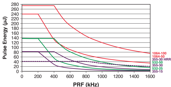
HyperRapid NXT Typical Single Pulse Energy Output
