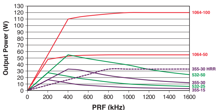
HyperRapid NXT Typical Power Output
